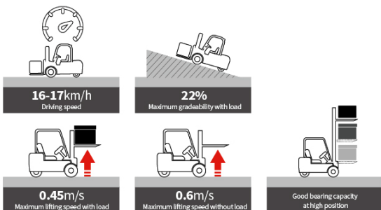
Front wheel dual drive motors provide more power.
